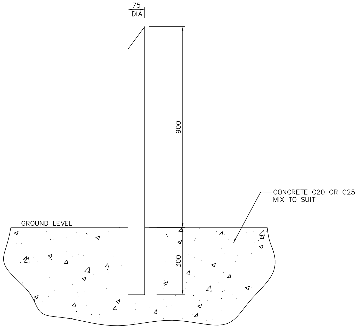
ALTO BOLLARDS CAPTAIN 75 DIA
